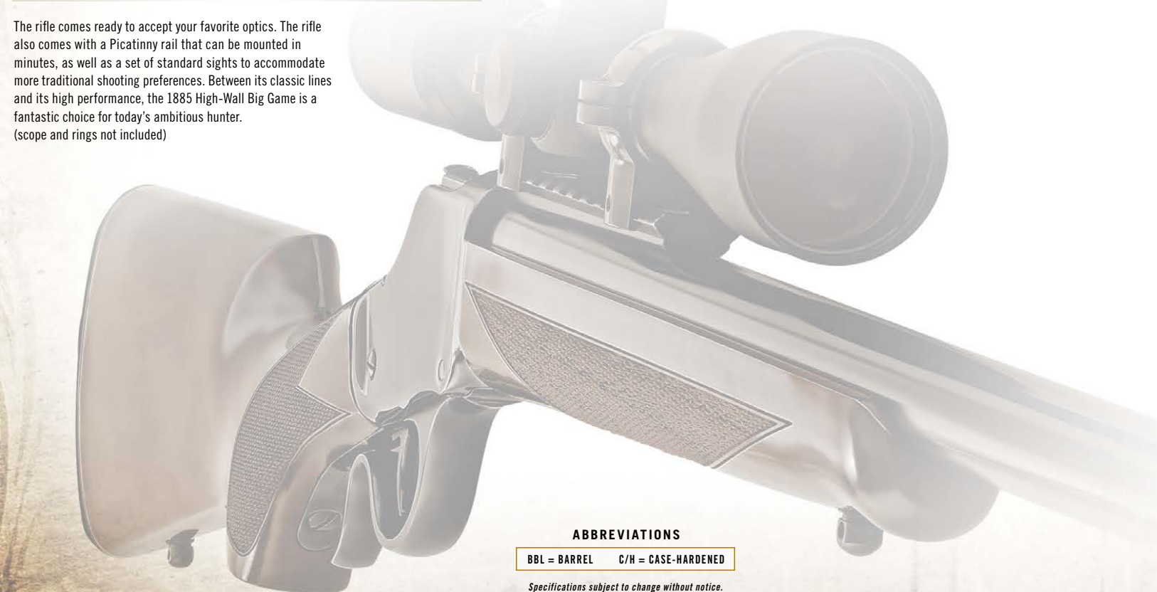
The 1885 High-Wall's loading lever (left), opens or locks the rifle's falling-block action (right).
